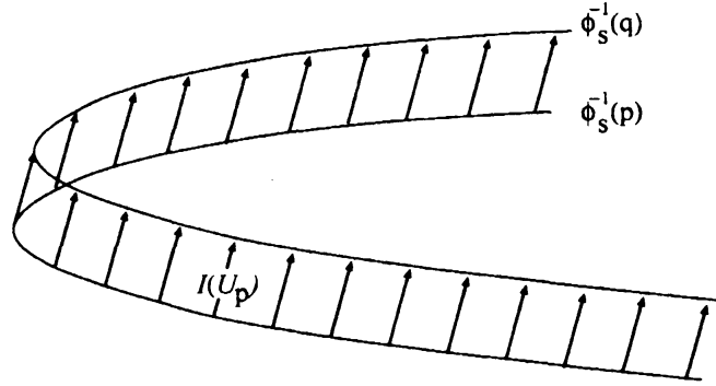
Figure 5: Morse Foliation
