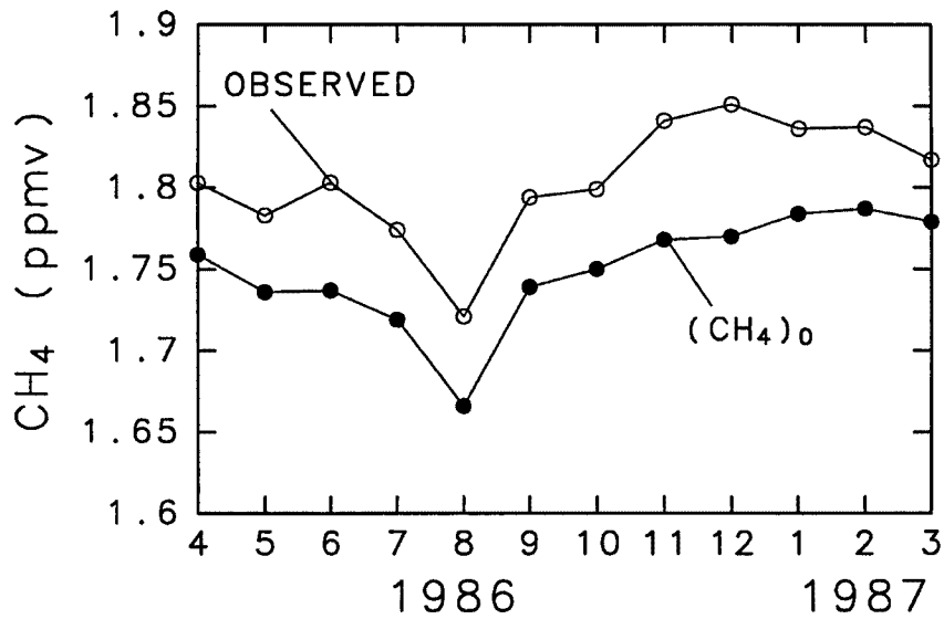
Fig. 7 Seasonal variations of observed and background (\text{CH}_4)_0 methane.
