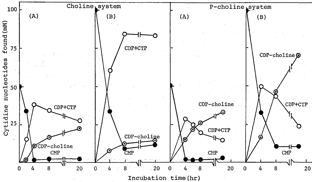
Fig. 6. Chemical changes in CDP-choline formation at high concentration of CMP. The reaction mixture contained (mM): glucose, 1200; phosphate buffer (pH 8.0), 300 in (A) or 400 in (B); \text{MgSO}_4 , 30; choline, 200 in choline system; P-choline in P-choline system. Dried cells, 200 mg per ml. Total volume 2.0 ml. Reaction was carried out by shaking at 28°C.
