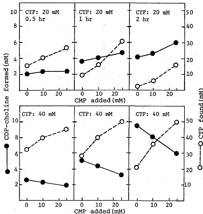
Fig. 7. Effect of supplied CMP on CDP-choline formation from CTP and choline. The reaction mixture contained (mM): glucose, 100; phosphate buffer (pH 8.0), 300; \text{MgSO}_4 , 30; choline, 80; CMP, indicated in the figures. Cells, 100 mg per ml. Shaken at 28°C in a total volume of 2 ml.
