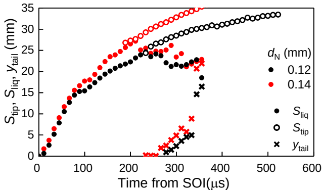
Figure 26. Effect of nozzle diameter on S_{tip} , S_{liq} , and y_{tail} with injection mass 0.50 mg and injection pressure 80 MPa (ambient temperature 850 K; ambient pressure 4 MPa).
