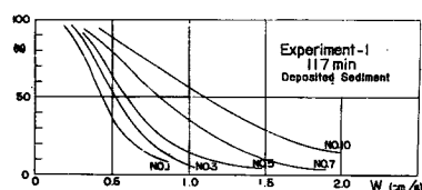
Fig. 7 Grain-size accumulation of deposited sediment.
