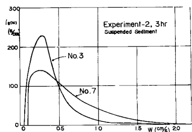
Fig. 9 Spectrum of fall-velocity distribution.
