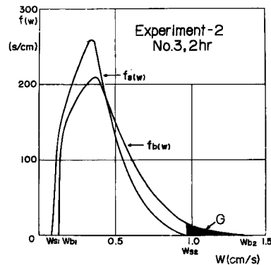
Fig. 12 Spectrum of fall-velocity distribution of suspended and deposited sediment.
