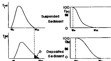
Fig. 11 Schematic diagram of grain-size accumulation of suspended and deposited sediment.
