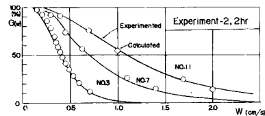
Fig. 13 Experimented and Calculated grain-size accumulation.
