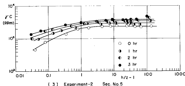
Fig. 6 Concentration of suspended sediment.
