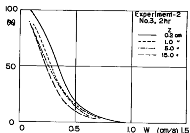
Fig. 10 Vertical variation of grain-size accumulation curve.
