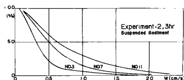
Fig. 8 Grain-size accumulation of suspended sediment.
