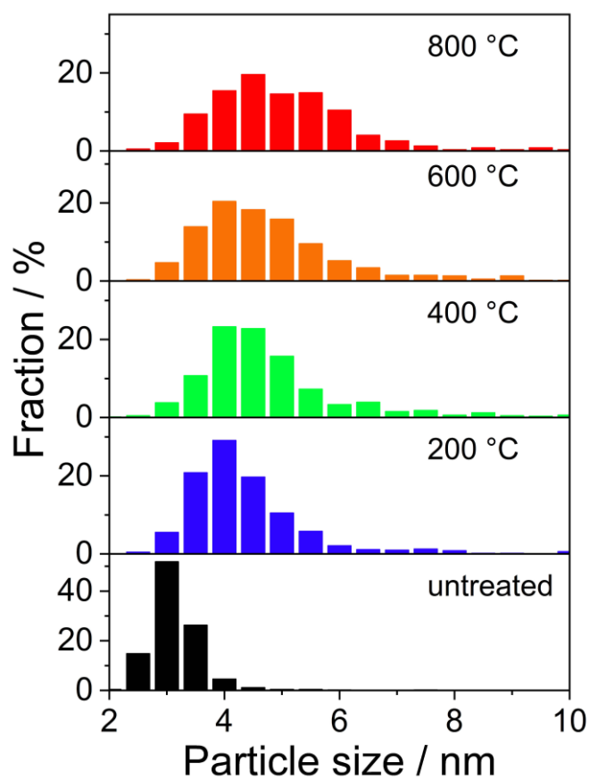
Figure 3. Particle size distributions of untreated and annealed samples. Black, blue, green, orange, and red sticks represent the untreated, 200, 400, 600, and 800°C of the annealing temperature, respectively
