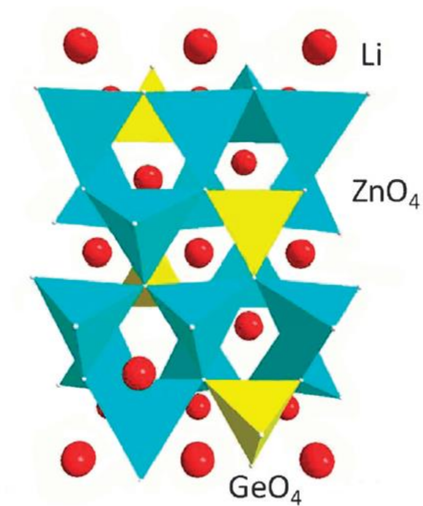
Figure 7. The crystal structure of The LISICON-like solid electrolyte using \text{Li}_{14}\text{Zn}(\text{GeO}_4)_4 as an example 49 .
