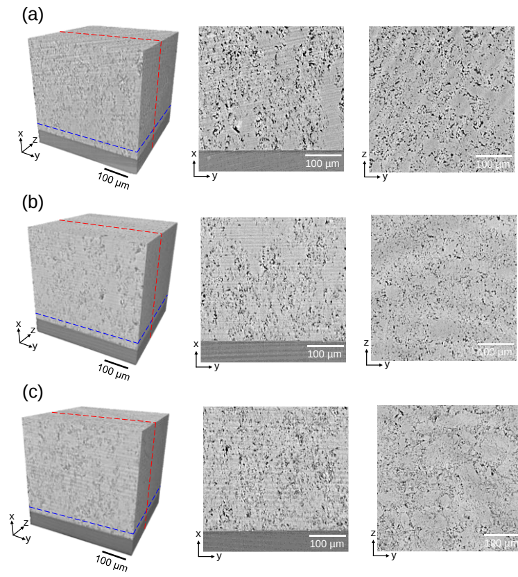
Figure 10. Transmission images of (a) Li 3 PS 4 , (b) unannealed 70Li 3 PS 4 -30LiI, and (c) 70Li 3 PS 4 -30LiI annealed at 200 °C before the galvanostatic cycling tests.
