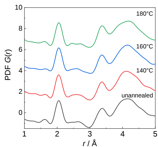
Figure 5. Reduced PDF, G(r) , of 70Li 3 PS 4 -30LiI prepared using the mechanical milling method before annealing and after annealing at various temperatures for 2 h.
