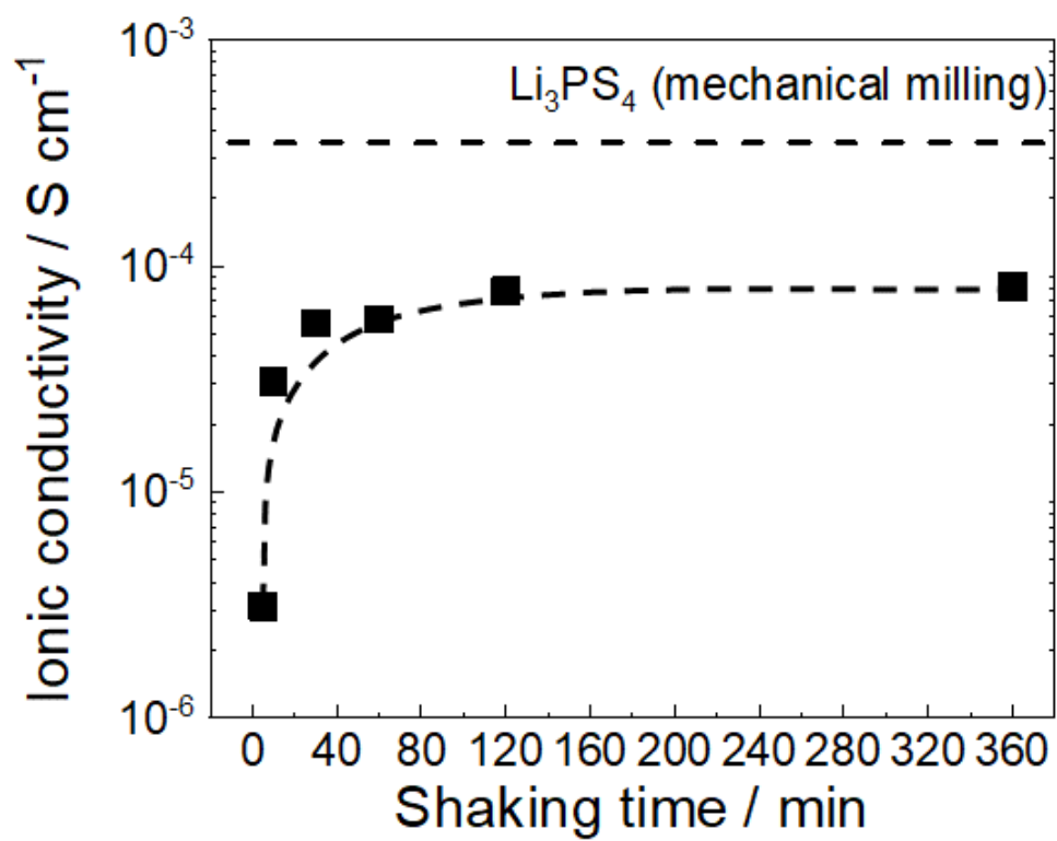
Figure 4. Correlation between the shaking time and the sample ionic conductivity after annealing at 170^\circ\text{C} for 2 h at 25^\circ\text{C} .
