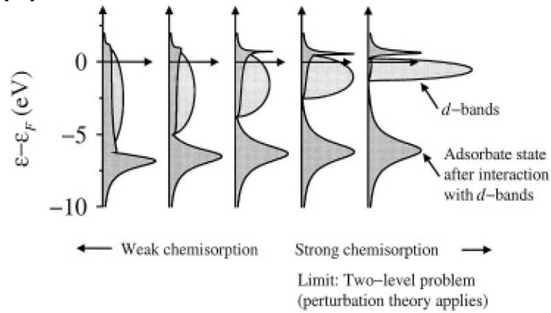
Figure 4. (a) Binding energies of atomic O vs d-band centers ( \epsilon_d ) of the four clean surfaces. (b) The local den sity of states proj ected onto an adsorbate state intera cting with the d bands at a surface 20 .
