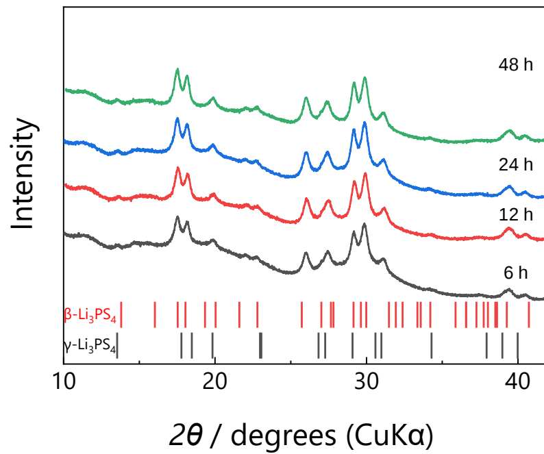
Figure 13. XRD patterns of samples annealed at 100°C for 6 h (black line), 12 h (red line), 24 h (blue line), 48 h (green line). Black bar is the reference material of \gamma -Li 3 PS 4 and red bar is the reference material of \beta -Li 3 PS 4 .
