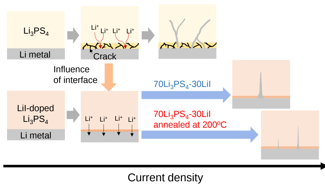
Figure 12. Schematic diagram of dendrite growth in Li 3 PS 4 and Li 3 PS 4 -LiI.
