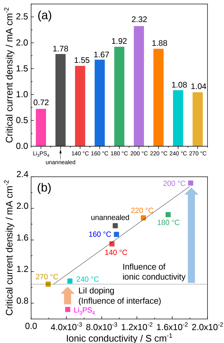
Figure 7. (a) Critical current densities at 100 °C of Li 3 PS 4 and 70Li 3 PS 4 -30LiI prepared using the mechanical milling method unannealed and after annealing at various temperatures for 2 h. (b) Correlations between the lithium ionic conductivity and critical current density at 100 °C of Li 3 PS 4 and 70Li 3 PS 4 -30LiI prepared using the mechanical milling method unannealed and after annealing at various temperatures for 2 h.
