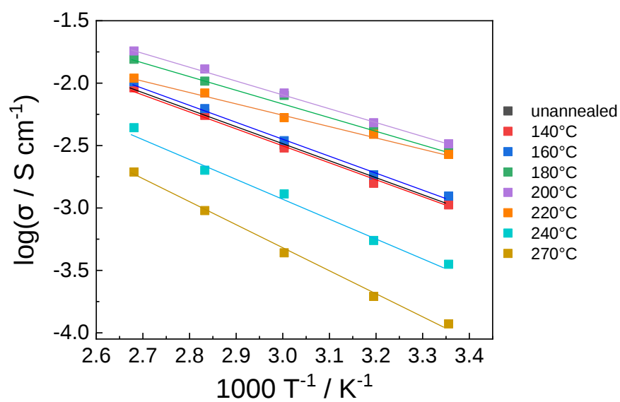
Figure 3. Arrhenius plots of 70\text{Li}_3\text{PS}_4\text{-}30\text{LiI} prepared using the mechanical milling method and annealed at various temperatures for 2 h.
