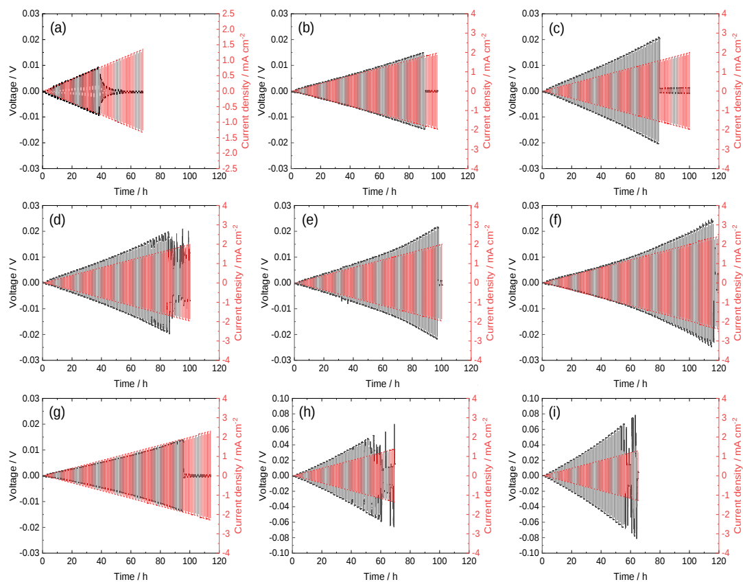
Figure 6. Galvanostatic cycling test results for (a) Li 3 PS 4 and 70Li 3 PS 4 -30LiI prepared using the mechanical milling method (b) unannealed and after annealing at (c) 140, (d) 160, (e) 180, (f) 200, (g) 220, (h) 240, and (i) 270 °C using the lithium metal/solid electrolyte/lithium metal cells with current density increasing by 0.04 mA cm -2 after charging and discharging for 1 h at 100 °C.
