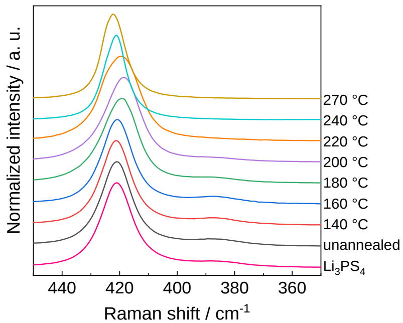
Figure 2. Raman spectra of \text{Li}_3\text{PS}_4 and 70\text{Li}_3\text{PS}_4\text{-}30\text{LiI} prepared using the mechanical milling method before annealing and after annealing at various temperatures.
