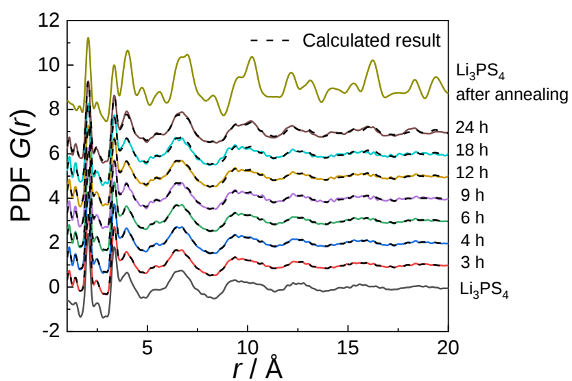
Figure 9. Results of PDF fitting of samples prepared using THF and annealed at 80^\circ\text{C} for different times.
