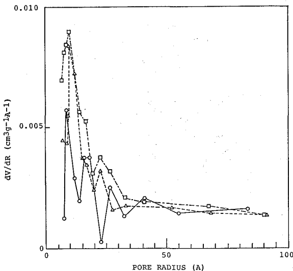
Fig. 4. Pore size distribution curves of the gels ( [\text{HCl}]/[\text{TMOS}] = 0.10 ) aged for different times at 40°C. Aged for 30 days (---□---), 45 days (---△---) and 120 days (—○—).
