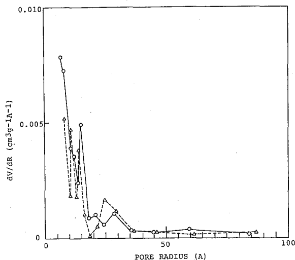
Fig. 5. Pore size distribution curves of the gels ( [HCl]/[TMOS] = 0.25 ) aged for 50 days at 40°C with (---Δ---) or without (—○—) exposure to water-saturated atmosphere for 2 days at 40°C.
