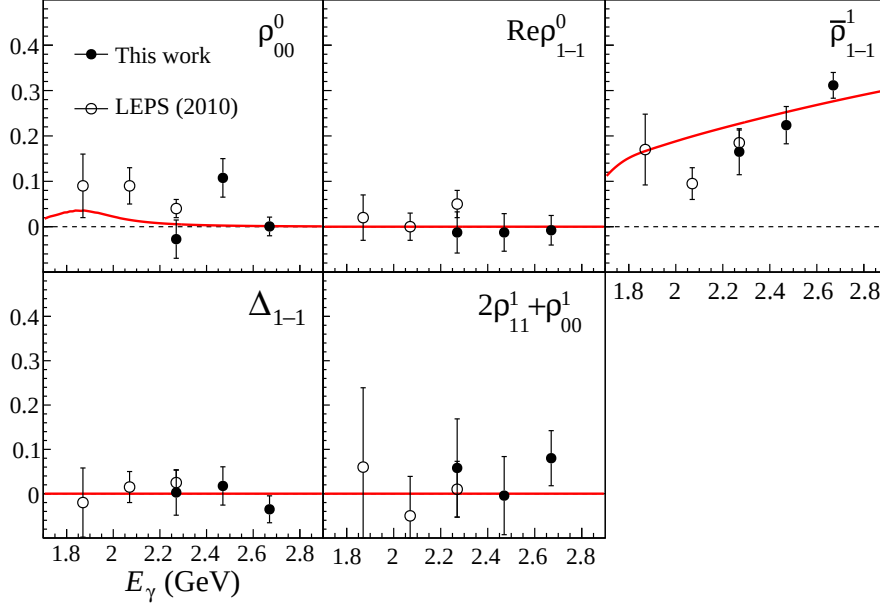
Fig. 5.10: E_\gamma dependence of spin-density matrix elements in the Gottfried-Jackson frame. The red solid curves represent the theoretical calculations at t = t_{\min} including the K^+\Lambda(1520) rescattering effect.
