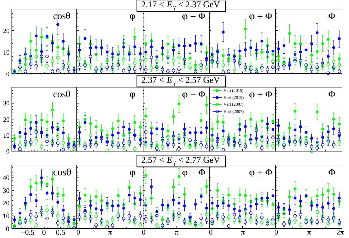
Fig. 3.14: Angle dependences of \phi -meson yields Y_{\phi \rightarrow K^+ K^-} (before acceptance correction) for t - t_{\min} > -0.05 \text{ GeV}^2 .
