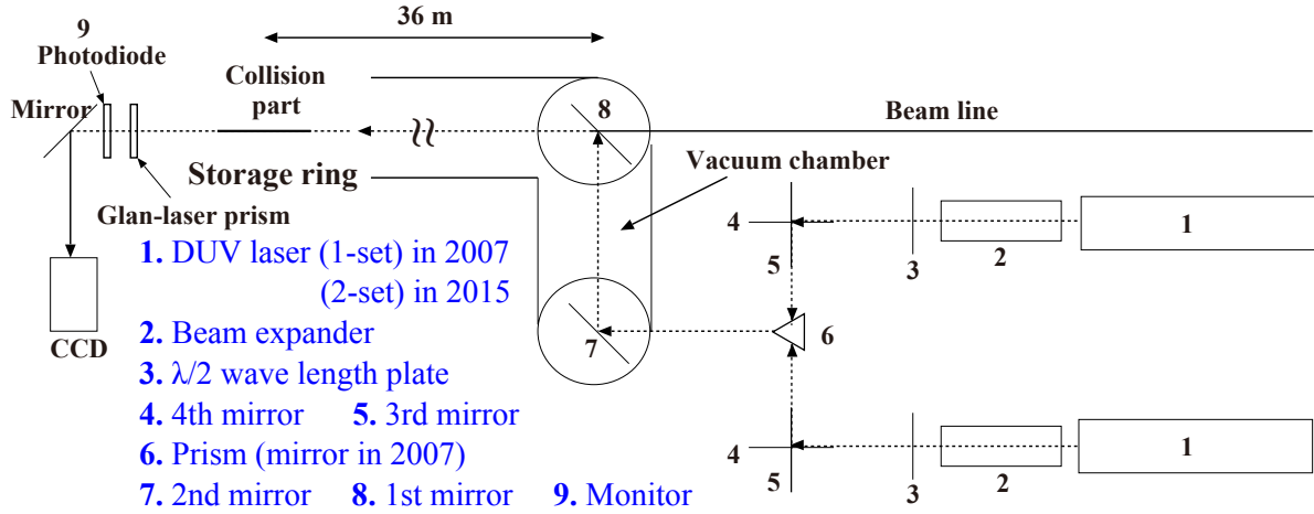
Fig. 2.4: Schematic view of the laser injection system.
