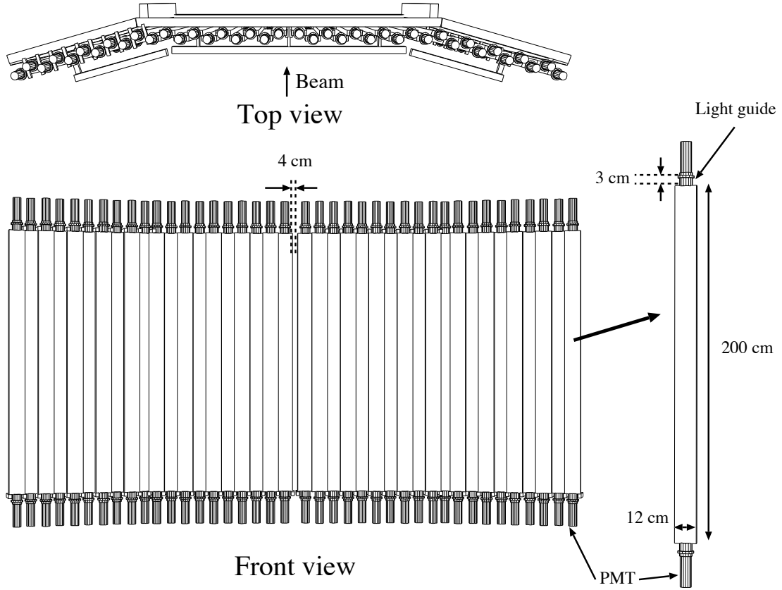
Fig. 2.19: TOF wall.
