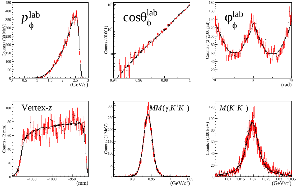
Fig. 3.16: Comparison between real data (red histograms) and MC results (black histograms). Top left: 3-momentum magnitude of \phi mesons in the laboratory frame. Top middle: Polar angle distribution of \phi mesons in the laboratory frame. Top right: Azimuthal angle distribution of \phi mesons in the laboratory frame. Bottom left: Vertex- z distribution of \phi mesons. Bottom middle: Missing mass distribution MM(\gamma, K^+K^-) . Bottom right: K^+K^- invariant mass distribution M(K^+K^-) after the background subtraction.
