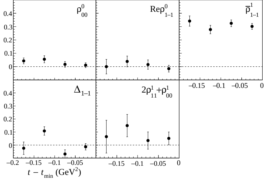
Fig. 4.14: t vs SDME results in the helicity system. The E_\gamma range is 2.37 < E_\gamma < 2.77 GeV.
