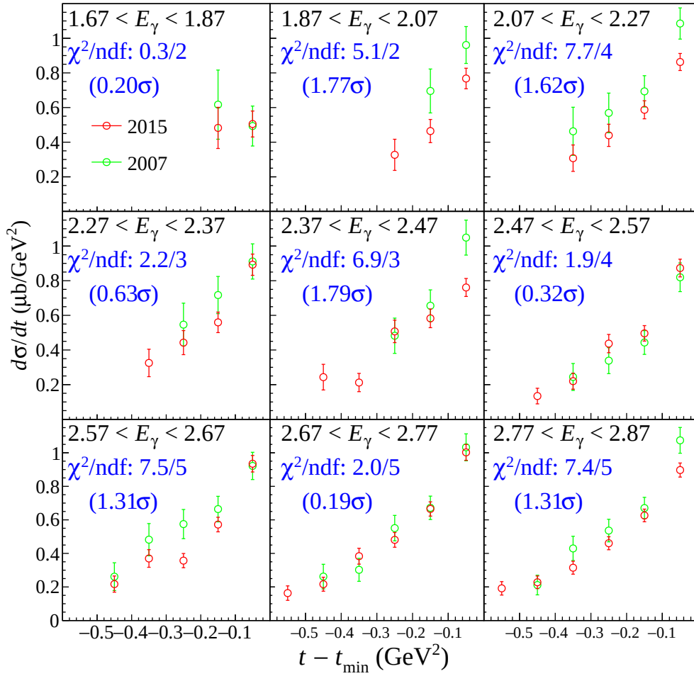
Fig. 4.1: t dependence of the differential cross sections d\sigma/dt for each E_\gamma bin. 2015 and 2007 results are compared. See text for details.
