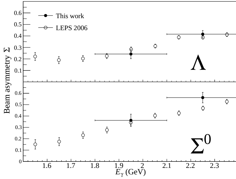
Fig. 3.27: Energy dependences of beam asymmetries. \cos \theta_{\text{c.m.}}^{K^+} > 0.6 . The top figure is for the \gamma p \rightarrow K^+ \Lambda reaction, and the bottom figure is for the \gamma p \rightarrow K^+ \Sigma^0 reaction. The open circles are taken from Ref. [66].
