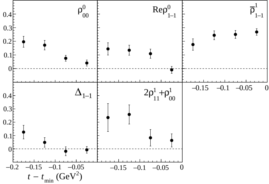
Fig. 4.13: t vs SDME results. The E_\gamma range is 2.37 < E_\gamma < 2.77 GeV.
