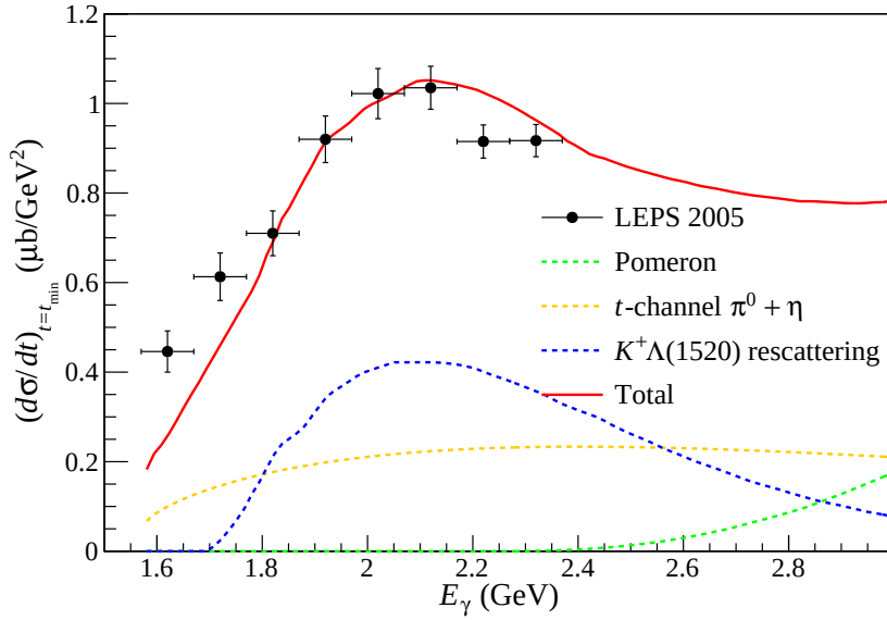
Fig. 1.25: Calculations of (d\sigma/dt)_{t=t_{\min}} including the rescattering amplitudes [47]. Only the dominant contributions are shown in the dashed lines. There are almost no contributions of Pomeron exchange amplitude (green dashed line) at low energies because of an artificial Pomeron suppression factor. See text and Ref. [47] for details.
