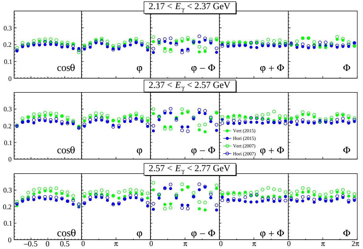
Fig. 3.18: Angle dependences of the acceptances for t - t_{\min} > -0.05 \text{ GeV}^2 .
