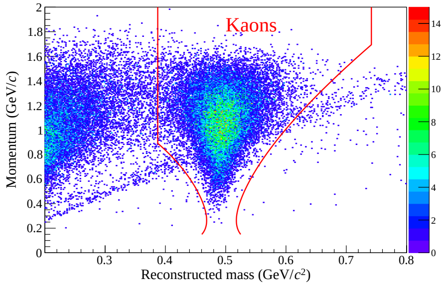
Fig. 3.3: Kaon identification. Two track events with opposite charge whose reconstructed masses are in the range of [0.2, 0.8] GeV/ c^2 (rough kaon selection) are plotted. The red boundary is the 4\sigma boundary. See text for details.
