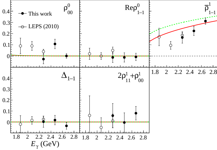
Fig. 5.6: E_\gamma dependence of spin-density matrix elements in the Gottfried-Jackson frame. The t range is t - t_{\min} > -0.05 GeV 2 . The open circles represent the previous LEPS results [10]. The red solid curves represent the theoretical calculations at zero degrees ( t = t_{\min} ) with the Pomeron strength factor C_{\mathbb{P}} determined by this work. The green dashed curves represent the same model with C_{\mathbb{P}} = 0.7566 GeV -2 [47].
