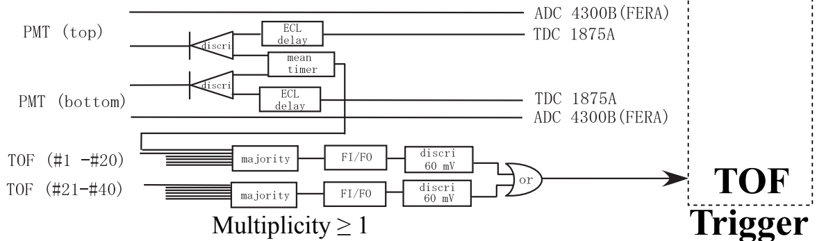
Fig. 2.21: Diagram of the readout circuits for triggers.
