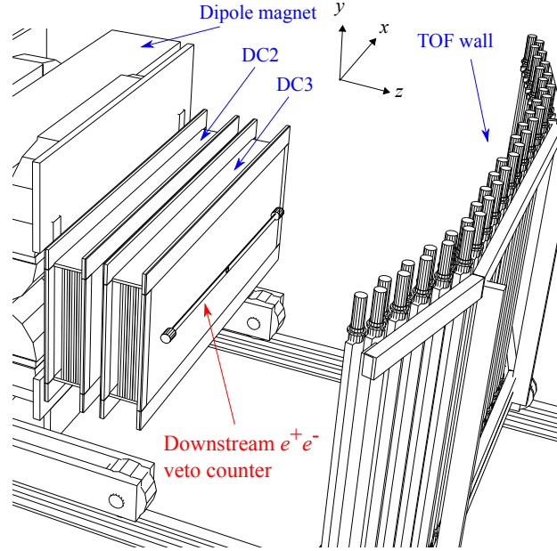
Fig. 2.17: Rear top view of the LEPS spectrometer.
