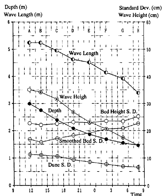
Fig. 8 (b) Time variation of dune height, dune length and water depth on Sept. 4-5, 1993
