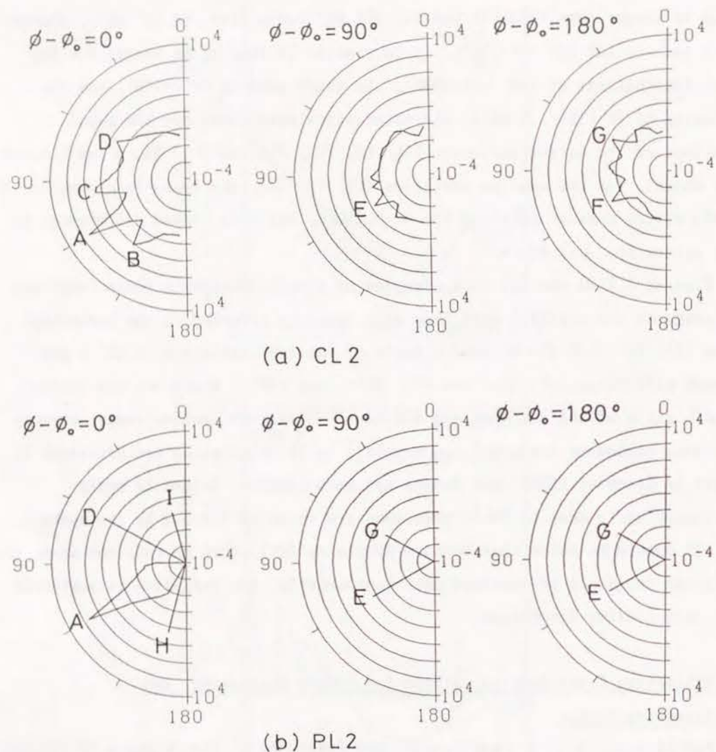
Fig.3.2 Phase functions of hexagonal ice crystals with long axes randomly oriented in the horizontal plane. (a) columns, (b) plates. \lambda=0.63\mu\text{m} . \theta_0=60^\circ , \phi-\phi_0=0^\circ, 90^\circ, 180^\circ . A:diffraction peak, B:upper tangent arc, C:lower tangent arc, D:subsun, E:parhelic circle, F:antehelion and parhelic circle, G:subparhelic circle, H:circumzenithal arc, I:subcircumzenithal arc.
