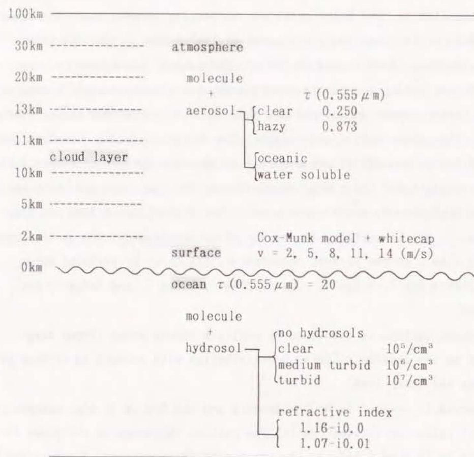
Fig.2.1 Diagram showing the atmosphere-ocean system.
