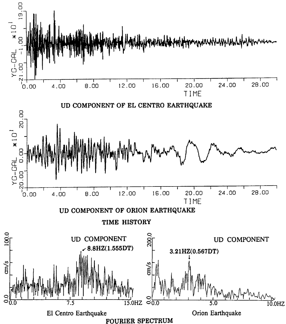
Fig. 7. Accelerograph and Fourier Spectrum of El Centro and Orion Earthquakes.
