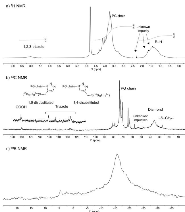
Figure 2. a) 1 H NMR, b) 13 C NMR by complete decoupling and c) 10 B NMR spectra of DND–PG( 10 B 12 H 11 2− )–COOH in D 2 O. The references are set at a) 4.80 ppm (the signal of HOD), b) 36.3 ppm (that of diamond core) and c) 19.49 ppm (that of 10 B(OH) 3 as an external standard).
