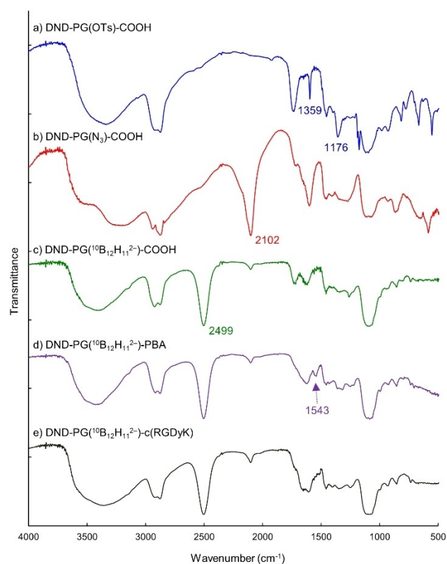
Figure 1. FT-IR spectra of BNCT nanodrugs and intermediates. a) DND–PG(OTs)–COOH, b) DND–PG(N 3 )–COOH, c) DND–PG( 10 B 12 H 11 2− )–COOH, d) DND–PG( 10 B 12 H 11 2− )–PBA, and e) DND–PG( 10 B 12 H 11 2− )–c(RGDyK).
