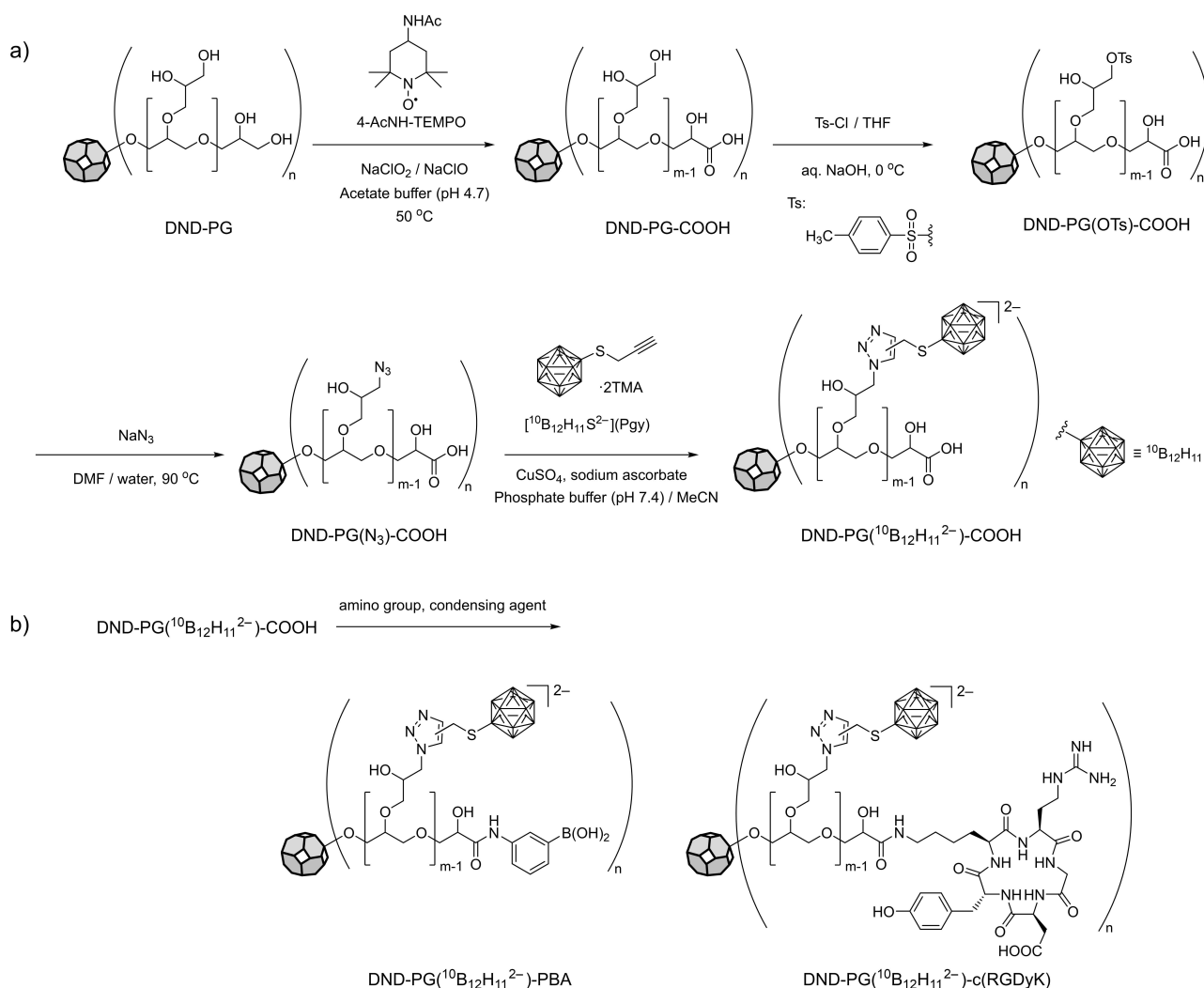
Scheme 1. Synthetic routes of BNCT nanodrugs starting from DND-PG. Introduction of a) ^{10}\text{B}_{12}\text{H}_{11}^{2-} moiety via Huisgen alkyne-azide cycloaddition (click reaction) at OH group and b) active targeting moieties through amide linkage at COOH group.
