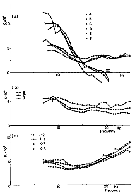
Fig. 20 Spring coefficients calculated from eq. (16).
