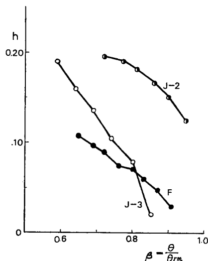
Fig. 18 Damping factor calculated from eq. (10).
