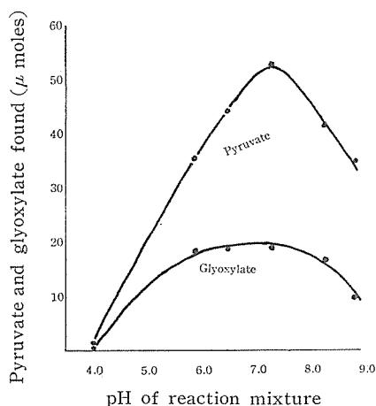
Fig. 1. Influence of pH on oxidation of glycollate and lactate by ammonium sulfate precipitates from Neurospora species.
