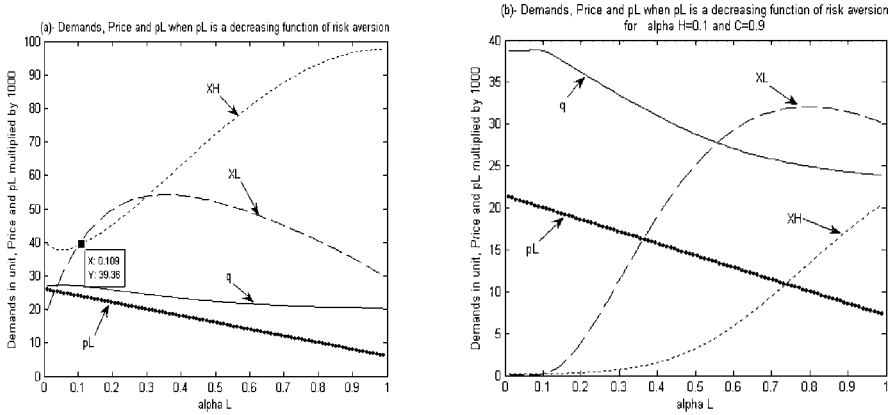
Figure 4 Demands, p_L and price when p_L is a decreasing linear function of \alpha_L :
