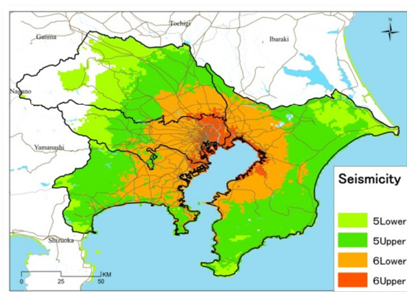
Fig.11 Seismic intensity
