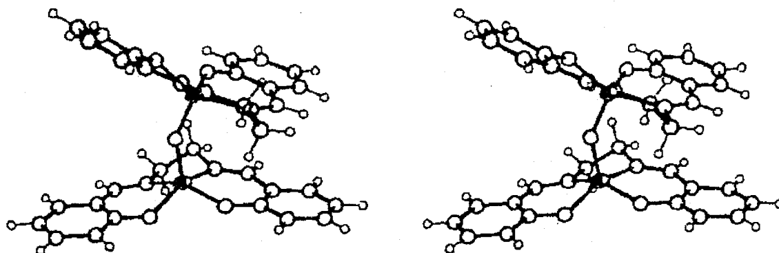
Figure 1. Stereoscopic illustration of the molecular geometry of [\text{Fe}(\text{salen})_2]\text{O} .
