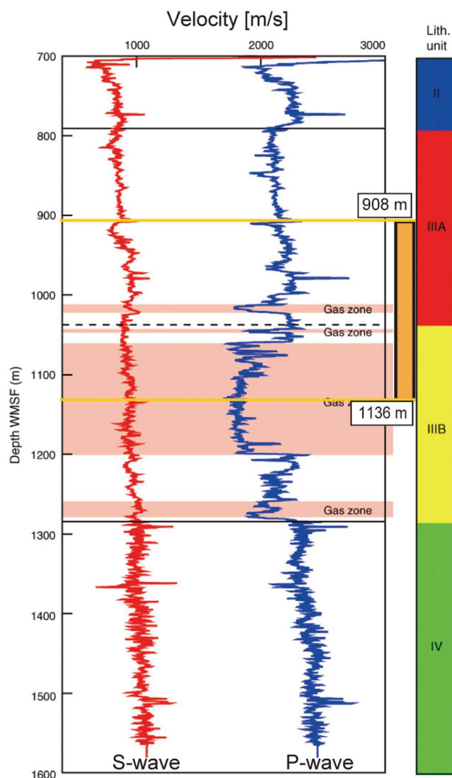
Figure 4. V_p and V_s estimated from downhole log data [Saffer et al., 2009]. The interval where the VSI tool was deployed is indicated by the orange bar. Lithologic units defined by the Expedition 319 Scientists [2010] are also shown.
