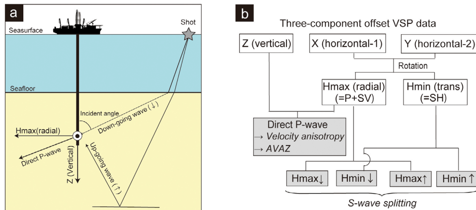
Figure 2. (a) Schematic image of the layout of the walkaround VSP survey. (b) Flow diagram illustrating wavefield separation. Gray boxes indicate the wavefields used for anisotropic analysis. From the direct P wave, we estimated P wave velocity anisotropy and amplitude variation with azimuth (AVAZ). From the horizontal components ( Hmax and Hmin ), we derived shear wave splitting.
