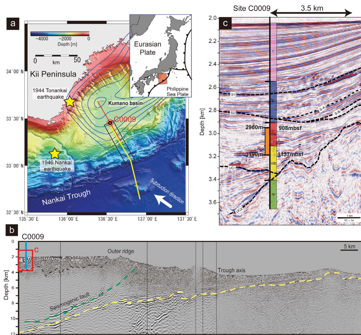
Figure 1. (a) Bathymetric map of the Nankai Trough around Site C0009. Red circle and line indicate the shooting tracks. Yellow line indicates the location of seismic profile displayed in Figure 1b. Black rectangle indicates the survey area of 3D seismic reflection data. Yellow stars mark the estimated hypocenters of the 1944 Tonankai earthquake (M 7.9) and the 1946 Nankai earthquake (M 8.0). Blue contours around the Kumano basin show the coseismic slip distribution of the 1944 Tonankai earthquake [Kikuchi et al. , 2003]. (b) Seismic profile across Site C0009. Yellow, green, and black dashed lines indicate oceanic crust surface, mega-splay fault, and base of the Kumano basin sequence, respectively. Red rectangle indicates the location of seismic profile displayed in Figure 1c. (c) Enlarged seismic profile across Site C0009. Lithologic units defined by the Expedition 319 Scientists [2010] are also shown. Orange bar shows the interval where the VSI was deployed.
