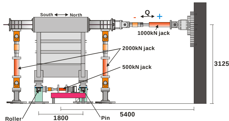
Fig.11 Loading System
