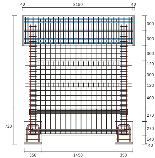
Fig.10 Reinforcing Details
