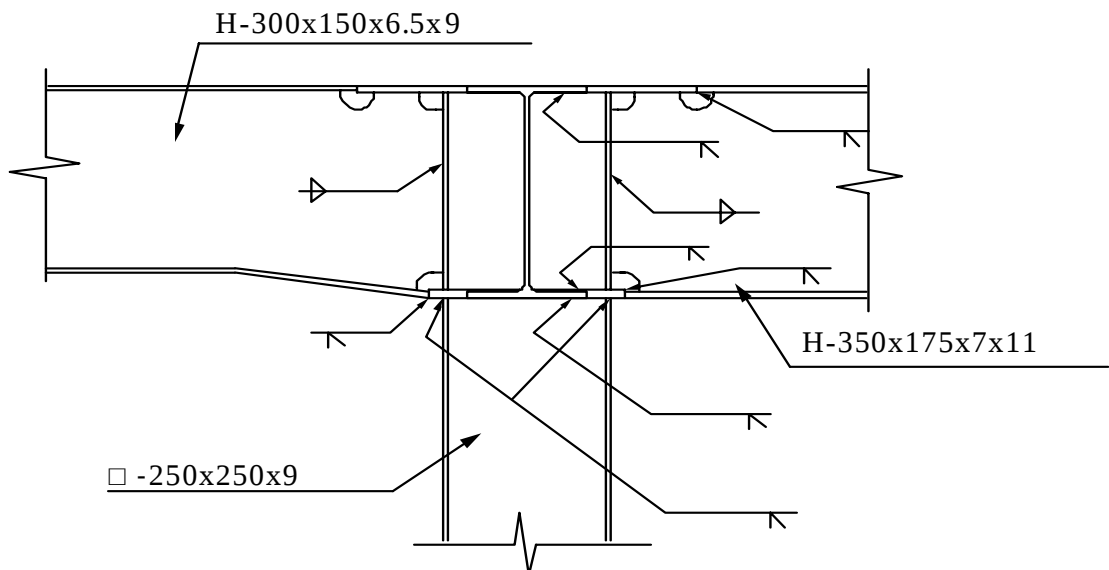
Fig. 5 Welded beam-to-column connection extracted from real structure
