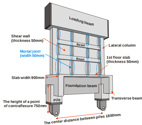
Fig.9 Perspective View of the Specimen
