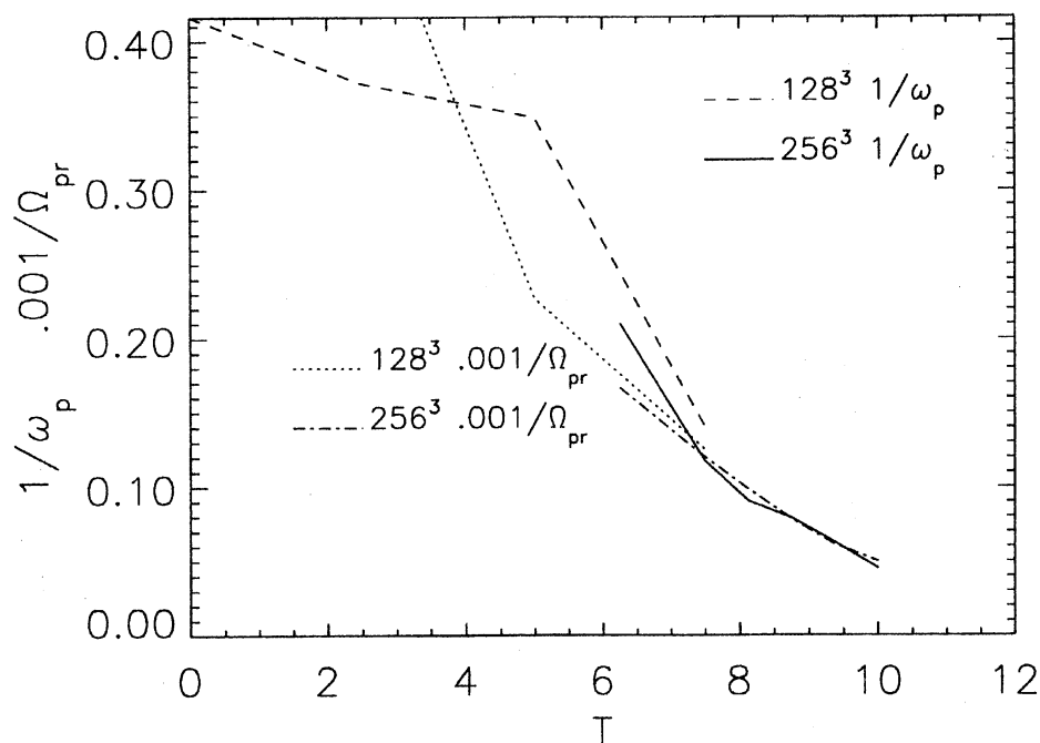
Figure 3: 1/||\omega||_\infty and 1/\omega_i e_{ij} \omega_j in Euler for orthogonal vortices.
