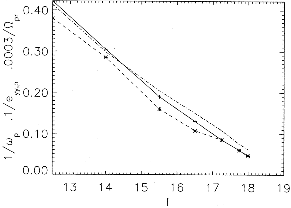
Figure 2: Dependence of 1/\|\omega\|_\infty , 1/\|e_{yy}\|_\infty and 1/\int dV \omega_i e_{ij} \omega_j on time from the anti-parallel Euler calculation [14] showing convergence to a singular time of about T = 18.7 .
