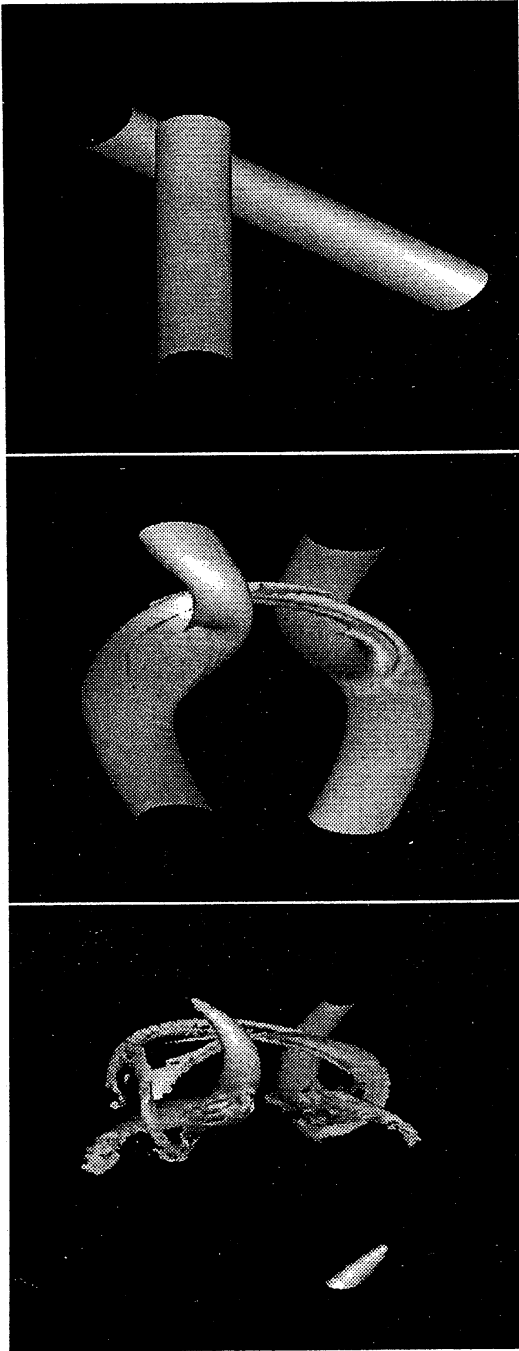
Figure 4: 1/\|\omega\|_\infty and 1/\omega_i e_{ij} \omega_j in Euler for orthogonal vortices. The three frames are t = 0, 6 and 10 . Arms are pulled out of the original vortices, become anti-parallel, then vorticity within the arms develops singular behavior.
