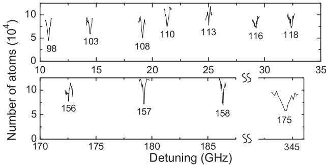
FIG. 1. Example of the observed spectra. The number of atoms after the PA laser irradiation is plotted as a function of the laser frequency detuning from the ^1S_0 \rightarrow ^1P_1 atomic resonance. The labels indicate the vibrational quantum numbers v' .
