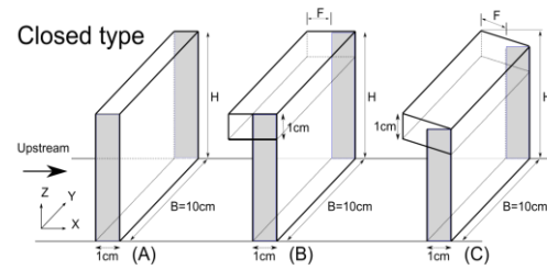
Fig. 4 Type of check dam
