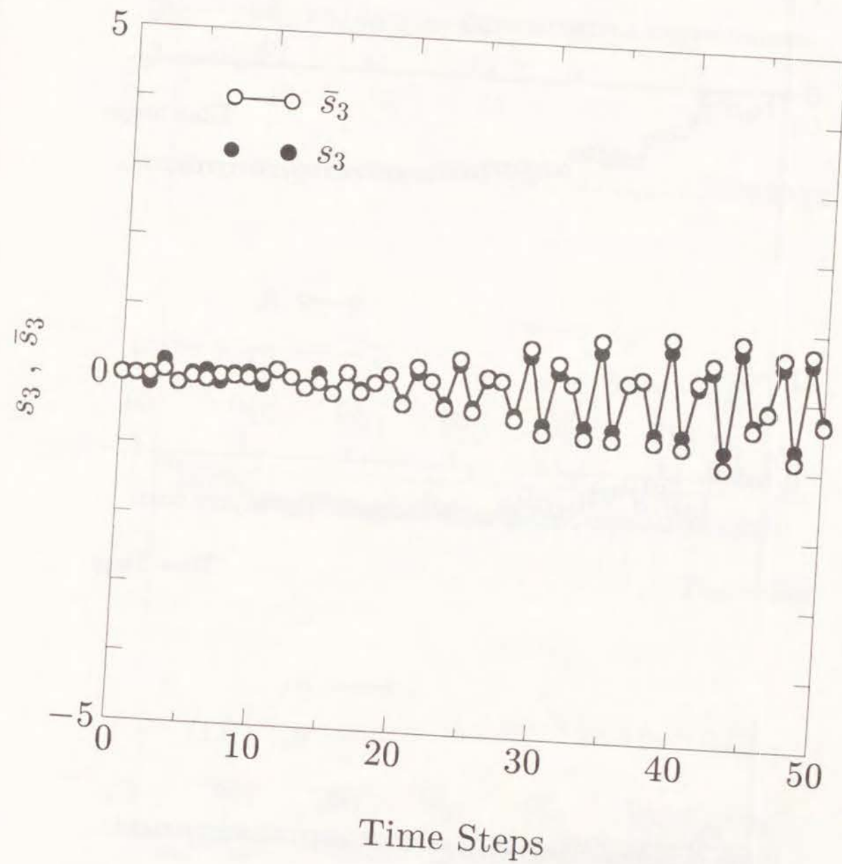
Figure 4.11: Estimation process of the disturbance s_3(k) of s(k) (Example 4.1).
