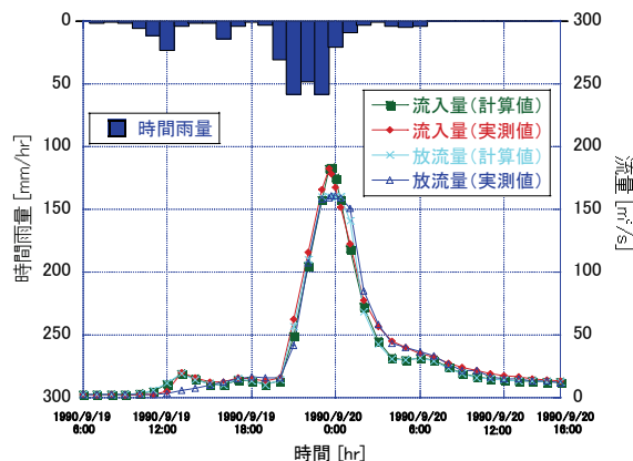
Fig. 6 The rainfall, observed/simulated inflow and outflow at the Hinogawa Dam during 19-20 Sep. 1990
