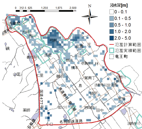
Fig.9 The simulated water depth (pattern 9) and digitized observed inundation areas
