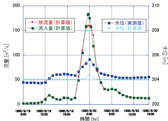
Fig. 7 The observed/simulated water stage at the Hinogawa Dam during 19-20 Sep. 1990
