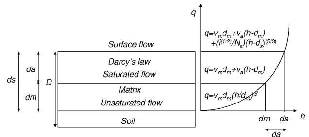
Fig. 5 The stage-discharge relationship
