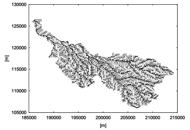
Fig. 4 The drainage path of the Hinogawa River catchment in the rainfall-runoff simulation
