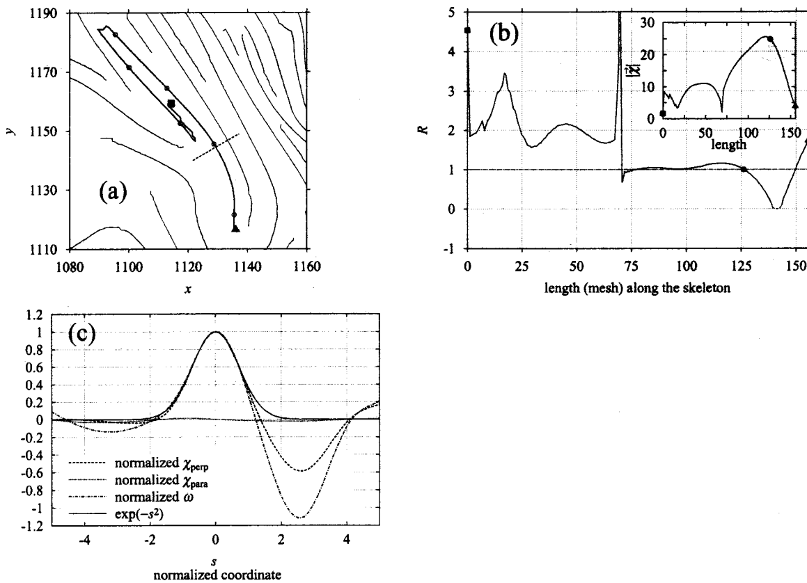
FIG. 6. (a) A tracked skeleton of a typical coherent structure obtained from the DNS with 2048^2 grid points. The length of the skeleton is 0.07 \times 2\pi . Open circles are marked at every other 25 mesh sizes along the skeleton from the end point marked with a filled square. (b) Deviation from the Burgers vortex layer solution along the skeleton. The end points marked with a filled square and triangle correspond to the same marks in (a). The ratio R is unity if T -vorticity and vorticity obey the Burgers vortex layer solutions. In the part denoted by the dotted line around (length)=135, the eigenvalue of the velocity gradient tensor becomes complex. Inset: the corresponding |\chi| along the skeleton. The spatial average of |\chi| in this snapshot is 8.1. This structure has a relatively large |\chi| value. (c) The behavior of T -vorticity and vorticity on the cut perpendicular to the skeleton, which is shown as the dashed line in Fig. 6(a) and the filled circle in (b). The plotted two component of T -vorticity, \chi_{\text{perp}} and \chi_{\text{para}} , are perpendicular and parallel component to the cut. The origin, s=0 , corresponds to the point on the skeleton. The coordinate s , T -vorticity \chi_{\text{perp}} , \chi_{\text{para}} and vorticity \omega are normalized with the values at the origin so that they collapse to \exp(-s^2) if they are the Burgers vortex layer solutions, Eqs. (23) and (24). The normalized unit length scale amounts to 0.96(2\pi/2048) . A width of the structure is hence estimated to be a few Kolmogorov dissipation scales (see Table I).
