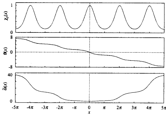
FIG. 17. A solution for \Psi(x) = -Ay \sin x : the T -vorticity, Eq. (58), the corresponding temperature \theta(x) and the response vorticity, Eq. (59). Here we set the parameters as A=1 , \kappa=1 , \alpha g=1 , \varphi=\pi/4 , \chi_0=1 , \theta(x=0)=0 and \tilde{\omega}_0=0 .
