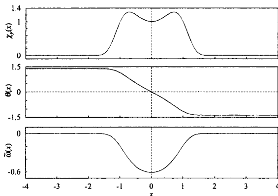
FIG. 15. The solutions for \Psi(x) = -Ay(4x^3 - 2x) : the T -vorticity Eq. (54), the corresponding temperature \theta(x) and the response vorticity, Eq. (55). Here we set the parameters as A=1 , \kappa=1 , \alpha g=1 , \varphi=\pi/4 , \chi_0=1 , \theta(x=0)=0 and \tilde{\omega}_0 = -e^{1/4}\sqrt{\pi}[1 + (2/\sqrt{\pi})\int_0^{1/2} e^{-\xi^2} d\xi]/(4\sqrt{2}) = -0.61 .
