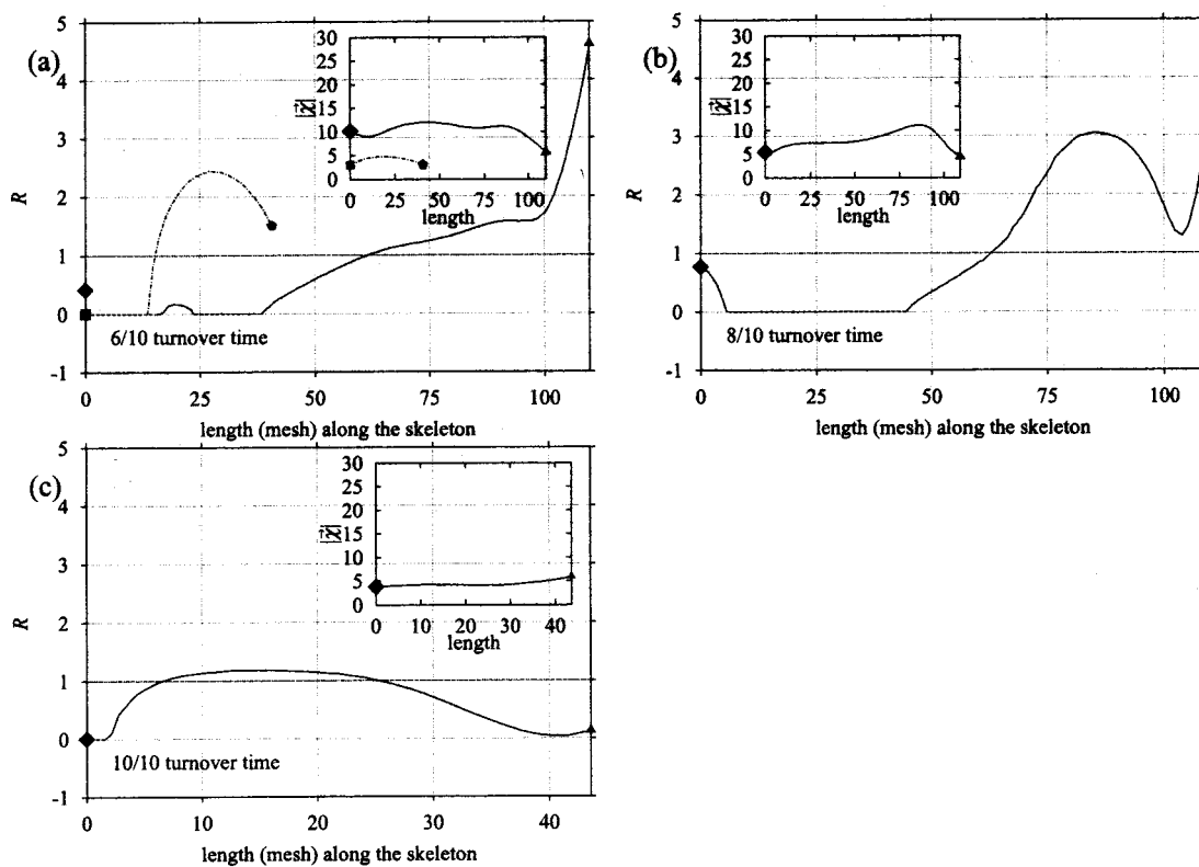
FIG. 12. The later stage evolution of the ratio R of the structure shown in Fig. 6. Insets: corresponding modulus of T -vorticity, |\chi| .
