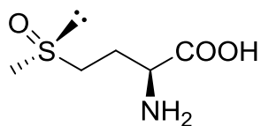
L-Methionine ( S )-sulfoxide
