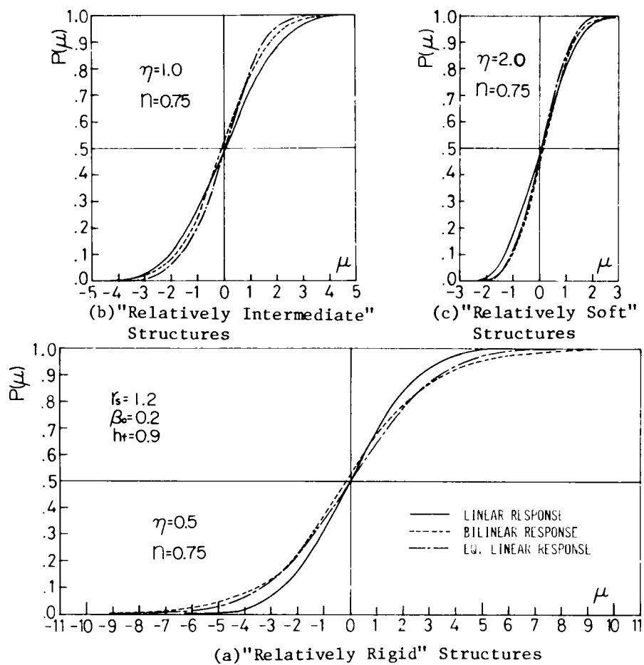
Fig.4.13 Simulated Probability Distribution of Ductility Factor (D.F.) Response of Linear, Bilinear( \eta=0.50 ) and Equivalent Linear Structures
