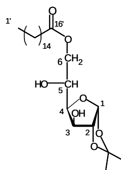
6- O -Palmitoyl-1,2- O -isopropylidene- α-D-glucofuranose 1
