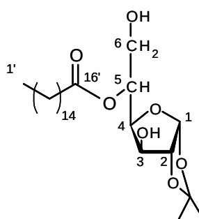
5- O -Palmitoyl-1,2- O -isopropylidene- α-D-glucofuranose 2
