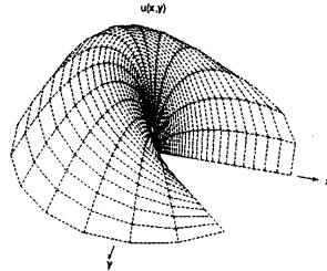
Fig 4: Solution for \alpha = 7\pi/4
