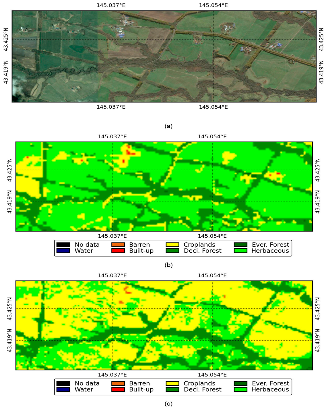
Figure 15. Performance of the JpLC-30 map over the JHR LULC map: (a) Google Earth™ image; (b) JHR LULC map; (c) JpLC-30 map.
