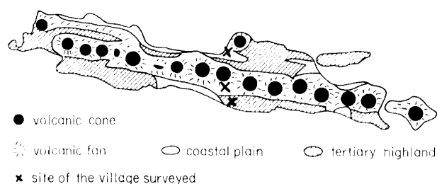
Fig. 1 Schematized geological framework of Java Island
