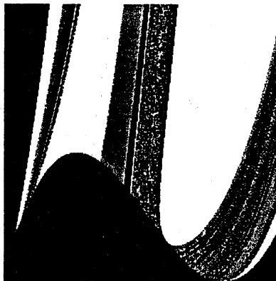
Figure 1: The connectedness locus C_3^R
