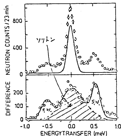
Upper: Observed inelastic spectrum at (0,0,1.9) at T=9.3 K and H=5 kG (circles). The full line is the observed profile at T=3.1 K and 30 kG which is assumed to be the background. Lower: Difference between the two spectra in the upper part of the figure. The full line is the result of a least-squares fit as described in the text.
