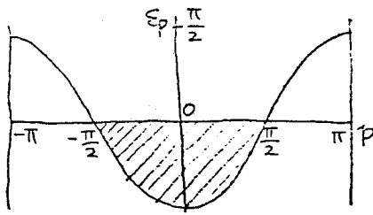
Ground state (Singlet)
