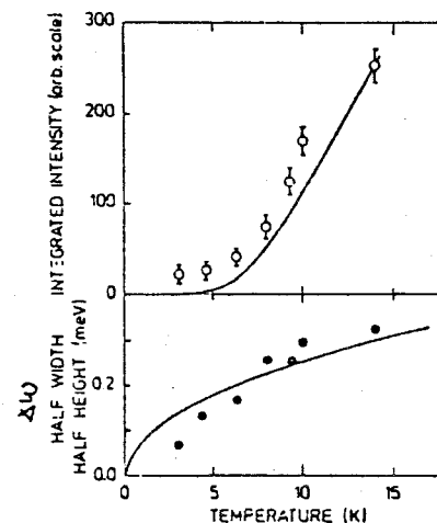
Temperature dependence of the integrated intensity (upper) and energy half-width at half-maximum (lower) of the quasielastic component at H=5 kG and q=(0,0,1.0) . The values are derived from the least-squares fitting procedure described in the text. The full lines are the results predicted by Mikeska with no adjustable parameter for the energy width and only a scale factor for the intensity.
