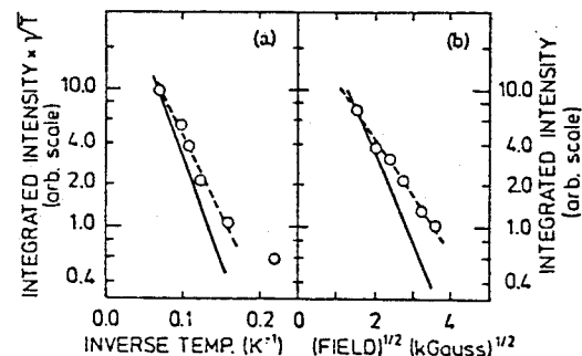
Semilog plots of the integrated quasielastic intensity at (0,0,1.9) vs inverse temperature at H=5 kG and (b) vs the square root of the field at T=9.5 K. The solid lines are calculated from the Mikeska theory.
