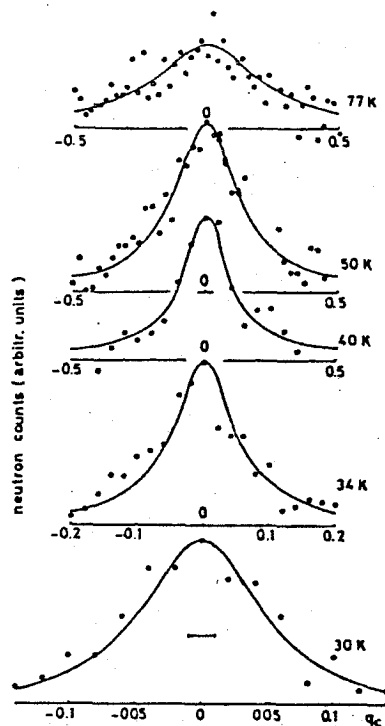
(b) The observed neutron scattering intensities for the q_c scan at different temperatures. The curves are the rigorous solutions for the corresponding temperatures. The resolution corrections are negligibly small as indicated by the width in the lowest figure.
