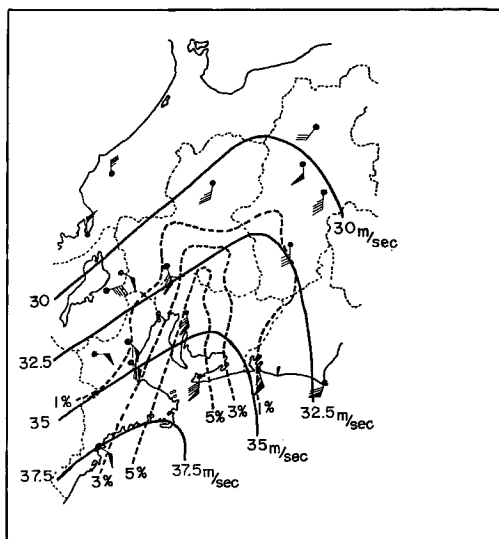
Fig. 5 Computed maximum wind speed (solid lines) and observed maximum wind speed (wind arrows) of Typhoon 5915. Dashed lines are the ratios of houses destroyed by wind
