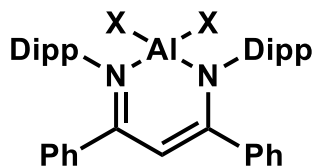
Fig. 1 Chemical structure of LAIH. (X = H, Dipp = 2,6-diisopropylphenyl).
