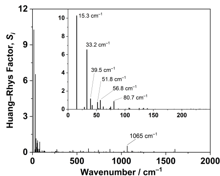
Fig. 2 Calculated Huang-Rhys factors for LAIH.
