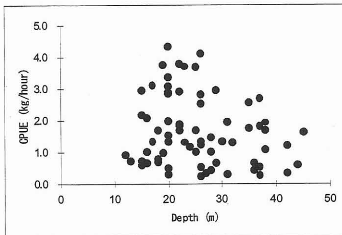
Figure 4. The vertical distribution of the shrimp distribution in the Gulf of Thailand 1996. The vertical axis means the CPUE (kg/hour) of each investigated point. The horizontal axis means the depth.
