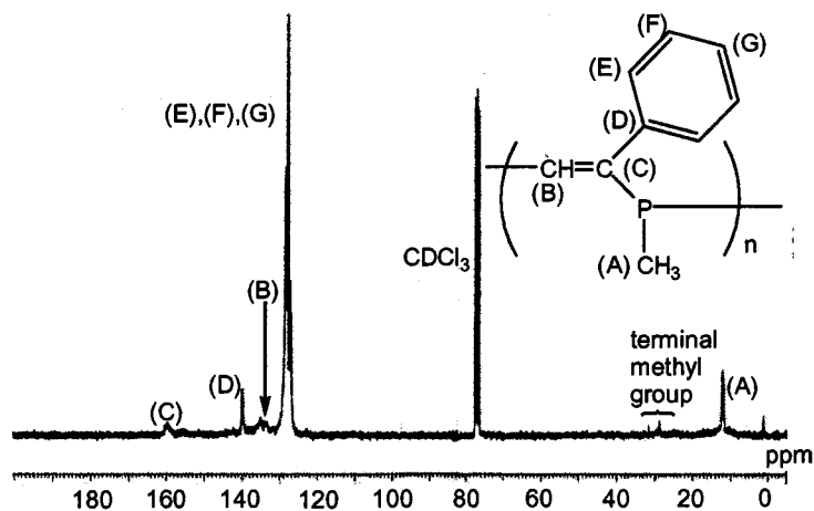
Figure 2. ^{13}\text{C} NMR spectrum of 1 .
