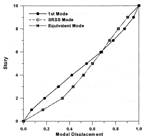
Fig. 5 Mode shapes
