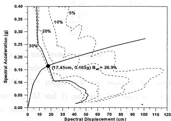
Fig. 11(c) Estimation of performance point (equivalent mode)
