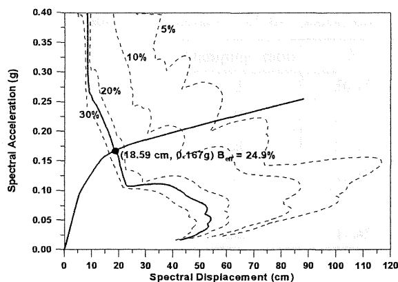
Fig. 11(a) Estimation of performance point (first mode)
