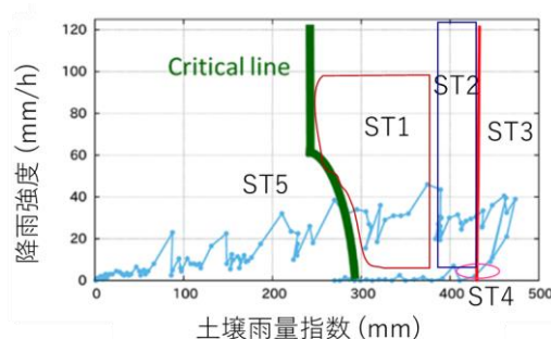
Fig.41 Multi-hazards at Shaolin Village by Typhoon MORAKOT
