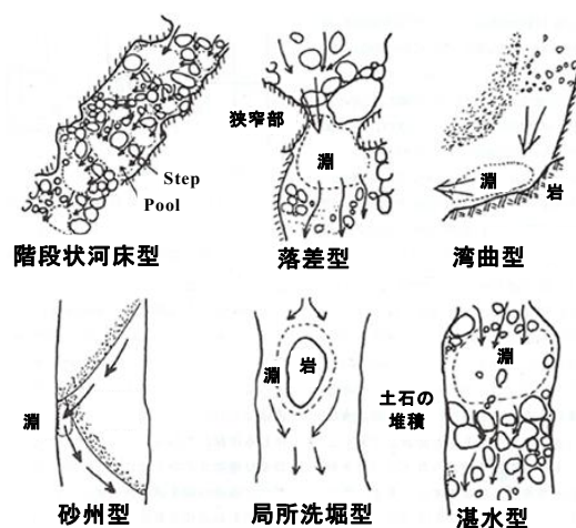
Fig.8 Classification of pools found in riverbed morphology
