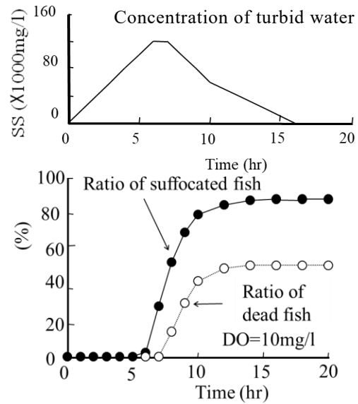
Fig.20 Suffocation rate and fatality rate of charrs due to turbid water
