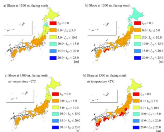
Fig.39 Freeze-thaw intensity on north-facing and south-facing slopes at a height of 1500 m in elevation (upper: Present temperature, lower: Present temperature + 2°C)
