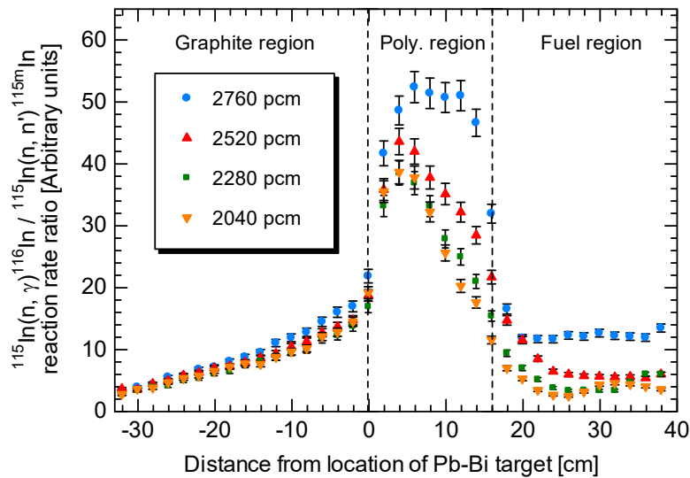
Fig. 5-2 Comparison between measured ^{115}\text{In}(n, \gamma)^{116m}\text{In} reaction rate distributions normalized by ^{115}\text{In}(n, n')^{115m}\text{In} along (13-14, A-Q) region shown in Figure 1.
