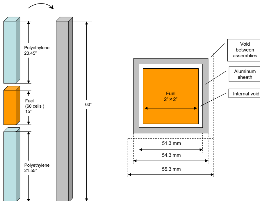
Fig. 1-2 Description of fuel assembly at KUCA
