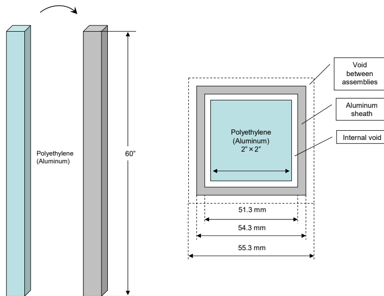
Fig. 1-5 Description of polyethylene reflector at KUCA
