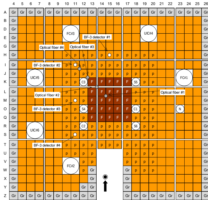
(a) Case 2-D (3000 HEU plates)
