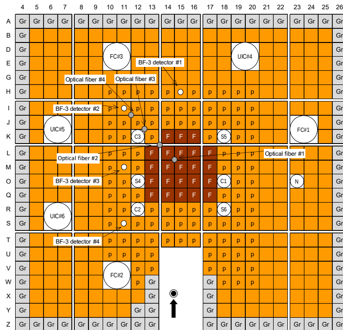
(b) Case 3-D (2760 HEU plates)
