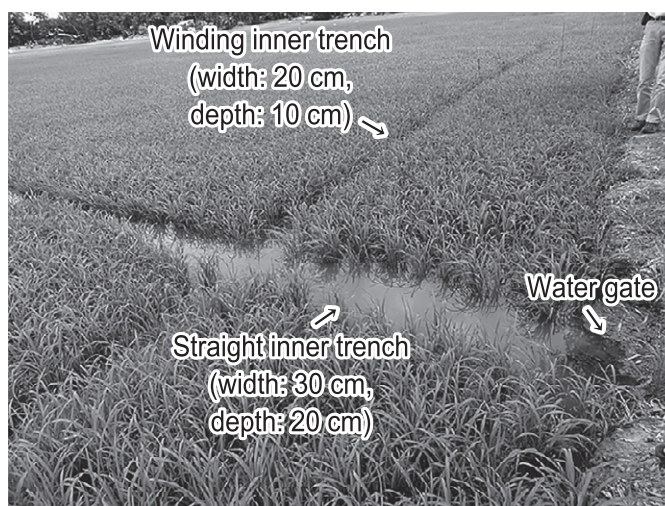
Fig. 8. Inner Trenches of a Paddy Field during the Rainy Season
