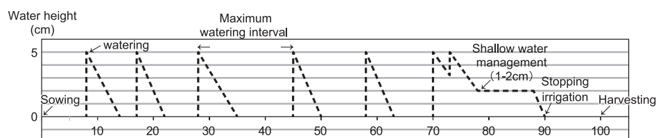
Fig. 2. Paddy Water Management during the Dry Season (taken from household A)
