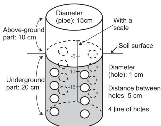
Fig. 6. Sketch of an Installed “Pani-pipe”
