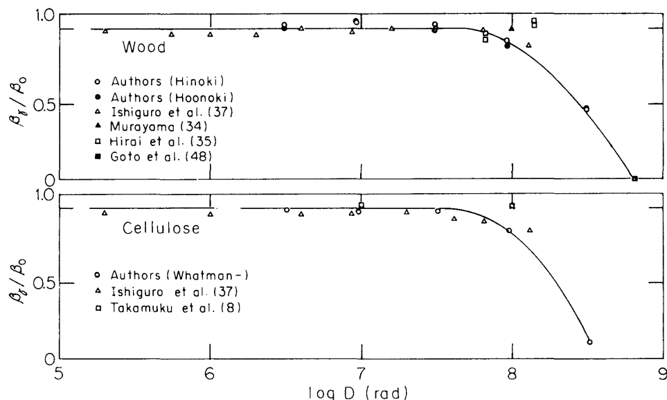
Fig. 3. Relative crystallinity index \beta_r/\beta_0 of wood and cellulose as a function of \log D .
