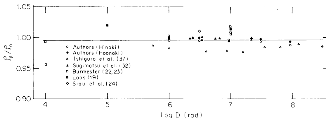
Fig. 2. Relative specific gravity \rho_r/\rho_0 of wood and cellulose as a function of irradiation dosage \log D . \rho_r : irradiated, \rho_0 : untreated.
