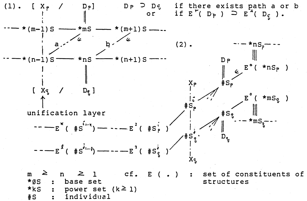
Fig.A2- Check diagram for D_P \supset D_Q
