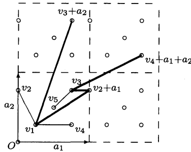
FIGURE 1. A graph \Gamma with \nu = 5 ; only edges of the fundamental graph \Gamma_f are shown; the bridges (v_1, v_2 + a_1) , (v_1, v_3 + a_2) , (v_3, v_2 + a_1) , (v_3, v_4 + a_1 + a_2) of \Gamma_f are marked by bold.
