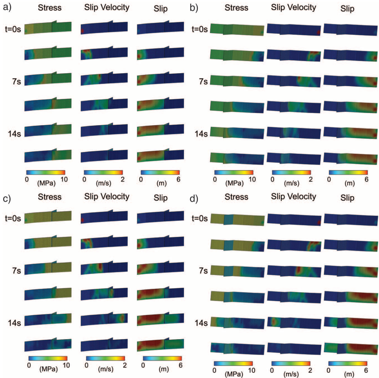
Figure 5. Results from numerical simulations with a 1.0 km gap between the northern edge of the buried fault segment (ce) and the southern edge of the surface-ruptured fault (bc). Snapshots of shear stress, slip velocity, and slip on the fault are shown at an interval of every 3.5 sec. (a) and (b) are for the case of \sigma_1 = N90^\circ E , and (c) and (d) are for the case of \sigma_1 = N105^\circ E . Cases (a) and (b) and cases (c) and (d) show the same results, respectively, as viewed from different directions, to see the whole rupture patterns. Scales are shown at the bottom of each sequence of snapshots. Note that the rupture propagates only on the Umehara fault (cd) but not on the Gifu-Ichinomiya line (ce) in the case of \sigma_1 = N90^\circ E (a) and (b), whereas it does not propagate on the Umehara fault (cd) but propagated on the Gifu-Ichinomiya line (ce) in the case of \sigma_1 = N105^\circ E (c) and (d).
