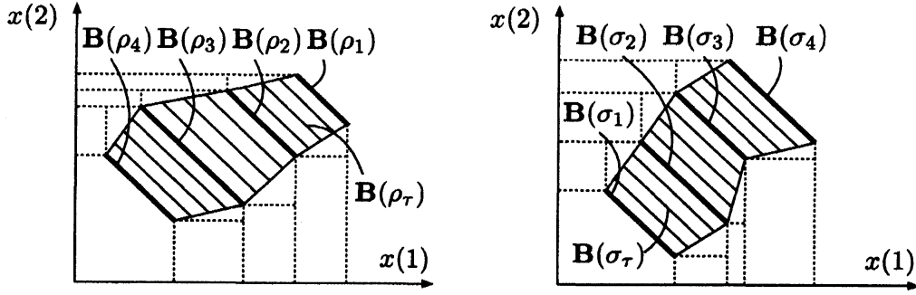
Figure 1: B(\rho_\tau) and B(\sigma_\tau) for all \tau \in [1, q]
