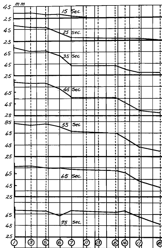
Fig. 33. Wave profile in Aji-River (case of initial water level O.P. +2.00m).
