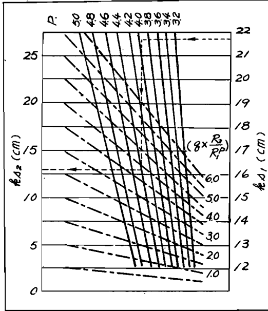
Fig. 7. k_{s1}-k_{s2} diagram. Abscissa is (k_{s1})^p . Full line: k_{s2}-(k_{s1})^p relation for constant p (the value of p in the diagram are erroneous. They must be divided by 10). Broken line; k_{s2}-(k_{s1})^p (relation for constant q . ( R_2/R_1^p )). Use of the diagram. Based on the values of k_{s1} , p and q . ( R_2/R_1^p ) obtained from Figs. 5 and 6, we proceed the path as indicated by the arrows, then the corresponding value of k_{s2} is obtained.
