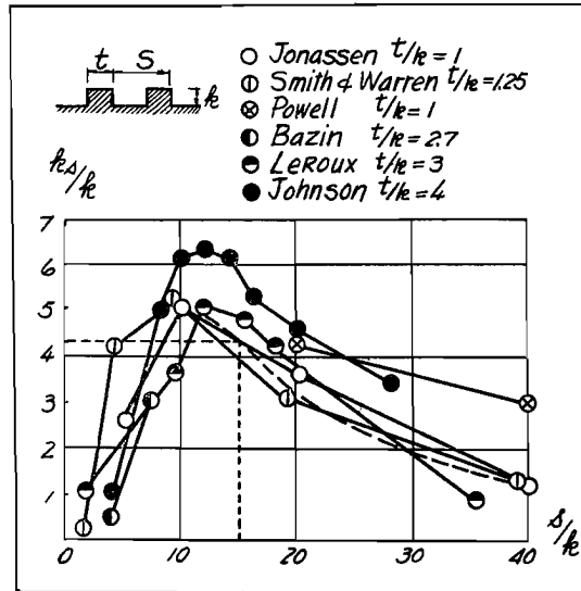
Fig. 8. k_s/k-S/k diagram.
