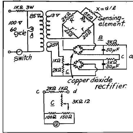
Fig. 11. Measuring circuit.
