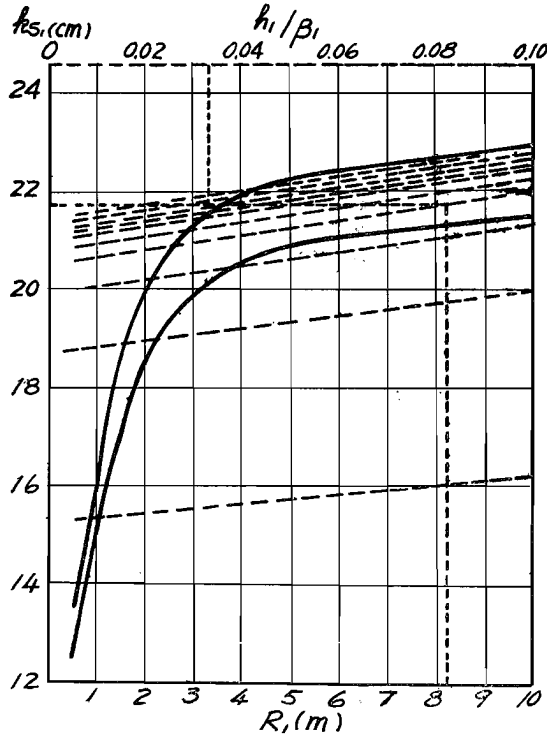
Fig. 5. Values of k_{81} corresponding to Manning's coefficient, n = 0.03 . Full line: equal h_1/B_1 -line, upper h_1/B_1 = 0.1 , lower h_1/B_1 = 0.005 . Broken line: equal R_1 -line, uppermost R_1 = 10 m, lowest R_1 = 1 m, interval of successive line = 1 m. Use of the diagram. Given R_1 or h_1/B_1 , then k_{81} is obtained on equal R_1 - or h_1/B_1 -line for any value of h_1/B_2 or R_1 .
