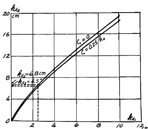
Fig. 27. Theoretical values of k_{s2} .
