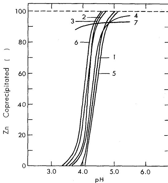
Fig. 4. Coprecipitation of zinc oxinate.
