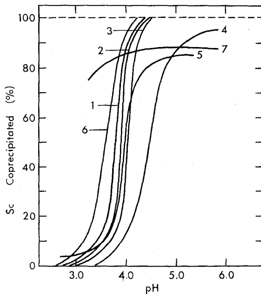
Fig. 3. Coprecipitation of scandium oxinate.
