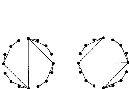
Figure 2: An optimal partitioning.
