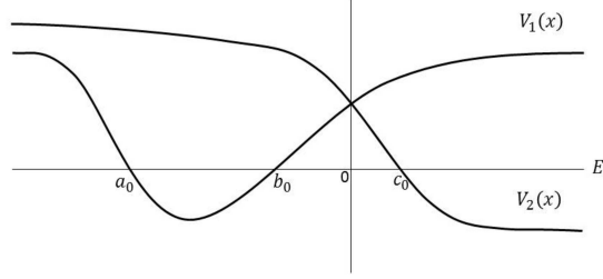
Fig. 1: The graph of the two potentials on the real axis
